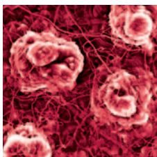
High-magnification SEM image of a ferrocene-treated silica layer after heating in flowing argon to ~1000 °C and exposure to methane for ~10 min Zhengjun Zhang et al 2003 Journal of Physics: Condensed Matter 15 L505–510
