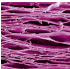
Scanning electron micrograph of a cross section of a ferroelectric film Xunlin Qiu et al 2005 Journal of Physics D: Applied Physics 38 649–654
