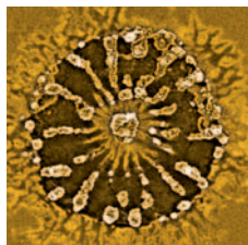
SEM image showing the surface morphology of a ferrocene-treated silica layer after heating to \sim 800^\circ\text{C} in flowing argon Zhengjun Zhang et al 2003 Journal of Physics: Condensed Matter 15 L505-510
